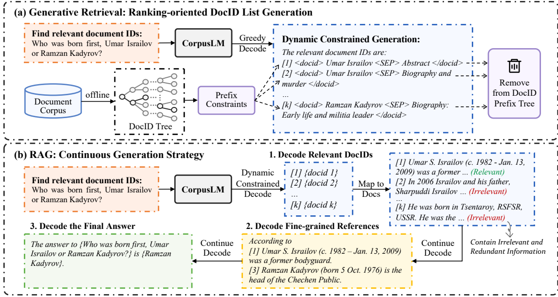
Figure 2: Illustration of the two generation strategies for retrieval and RAG. (a) Ranking-oriented DocID list generation strategy. We utilize a prefix tree built from DocIDs in the corpus to dynamically add constraints for generating valid and non-repeated DocID ranking list. (b) Continuous generation strategy. It comprises three continuous decoding steps: (1) decode DocIDs and map them to the corresponding documents; (2) decode fine-grained references from the documents; (3) decode the final answer.
